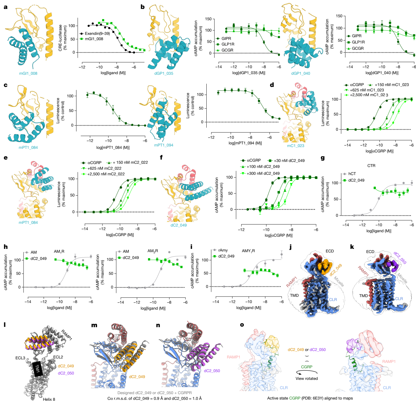
Fig. 4 | Characterization of class B GPCR miniprotein antagonists.
