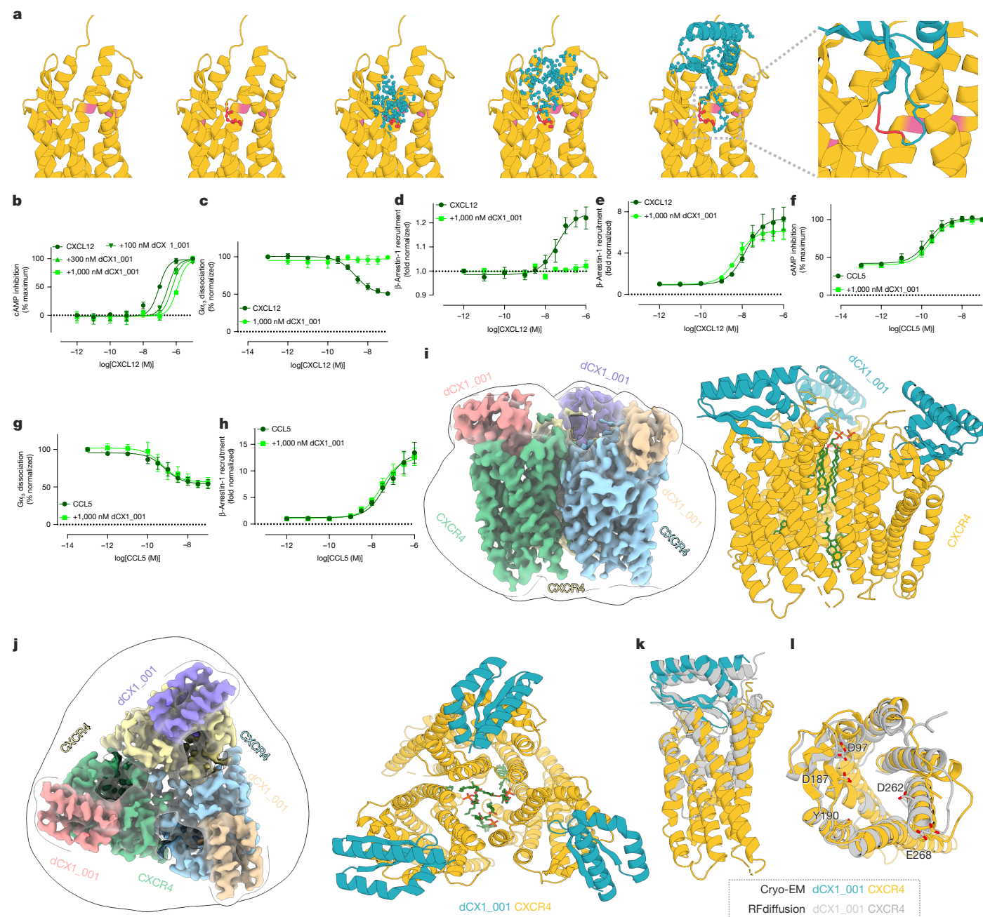
Fig. 3 | Pharmacology and cryo-EM structure of a designed CXCR4 antagonist. a , A representative RFdiffusion trajectory for generating binders (blue) against CXCR4 (yellow; PDB: 4RWS). Selected hotspots are highlighted in pink and de novo pentamer motifs used for scaffolding are shown in red. Inset: deep insertion of the motif (red) and the resulting binder. The receptor structure was truncated for clarity. b , Functional cAMP assay of the dCX1_001 binder in CHO cells stably expressing CXCR4. Data are mean \pm s.e.m. n = 4 biological replicates. Schild regression analysis indicates that dCX1_001 is an antagonist with a pA_2 of 7.6 \pm 0.3 (25 nM) and a slope of 0.68 \pm 0.13 . c , Inhibition of G protein activation by dCX1_001 binder at CXCR4 in a NanoBiT-based G\alpha_{13} dissociation assay. Data are mean \pm s.e.m. n = 3 biological replicates. d, e , \beta -Arrestin-1
