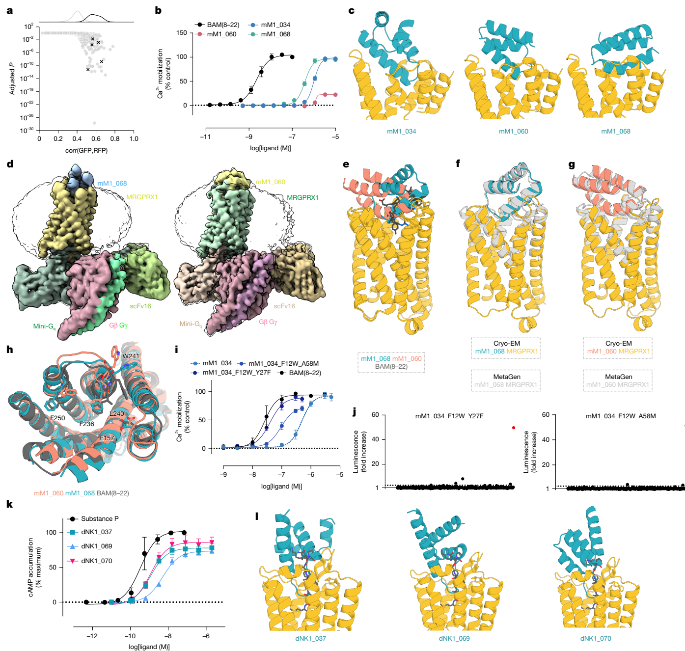
Fig. 2 | Characterization of MRGPRX1 and NK1R agonists. a , In total, 13,000 MetaGen-designed MRGPRX1 agonists were tested using OPS-RD. The colocalization (binding signal) induced in cells with the same binder was compared to the colocalization distribution across all imaged cells (over 2.5 million). P values were computed using a one-sided Kolmogorov–Smirnov test and adjusted using the Benjamini–Hochberg procedure. P values are provided in the MRGPRX1 dataset (Data availability). Functional hits are indicated by a ‘x’ symbol. b , Concentration–response curves of agonist hits and positive control BAM(8–22) in a calcium flux assay. Data are mean \pm s.e.m. n = 3 (mM1_034, mM1_060, mM1_068) and n = 4 (BAM(8–22)) biological replicates. c , Computational models of three agonist hits (receptors truncated for clarity). d , Cryo-EM maps of mM1_068 (left) and mM1_060 (right) bound to MRGPRX1 (the low-threshold map indicates detergent micelles). e , Alignment of mM1_068, mM1_060 and BAM(8–22) cryo-EM models bound to MRGPRX1. f, g , Alignment of cryo-EM structures of mM1_068 (f) and mM1_060 (g) bound
