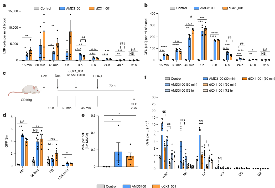
Fig. 5 | Mobilization of HSPCs by dCX1_001 and AMD3100. Human CD46-transgenic mice were injected subcutaneously with PBS (control), AMD3100 (5 mg per kg) or dCX1_001 (5 mg per kg). Blood samples were collected at the indicated timepoints. a , Flow cytometry quantification of LSK cells. Data are mean \pm s.e.m. n = 5 mice per group. Statistical analysis was performed using two-sided two-way ANOVA with Šidák's multiple-comparison test. Asterisks (control versus ligand) and hashes (dCX1_001 versus AMD3100) indicate statistical significance; * P \leq 0.05 , ** P \leq 0.01 , *** P \leq 0.001 , **** P \leq 0.0001 , ## P \leq 0.01 , ### P \leq 0.001 ; NS, not significant. b , Colony-forming assay of white blood cells (WBCs) plated in cytokine-supplemented, semi-solid medium; colonies were counted after 10 days. Data are mean \pm s.e.m. n = 5 mice per group. Statistical analysis was performed as in a ; # P \leq 0.05 . c , Schematic of in vivo mobilization and HSPC transduction. Mice received dexamethasone (dex) (16 h and 1.45 h) followed by AMD3100 or dCX1_001 (45 min) and intravenous HDAd injection; tissues were collected after 72 h. d , GFP expression in total mononuclear cells
