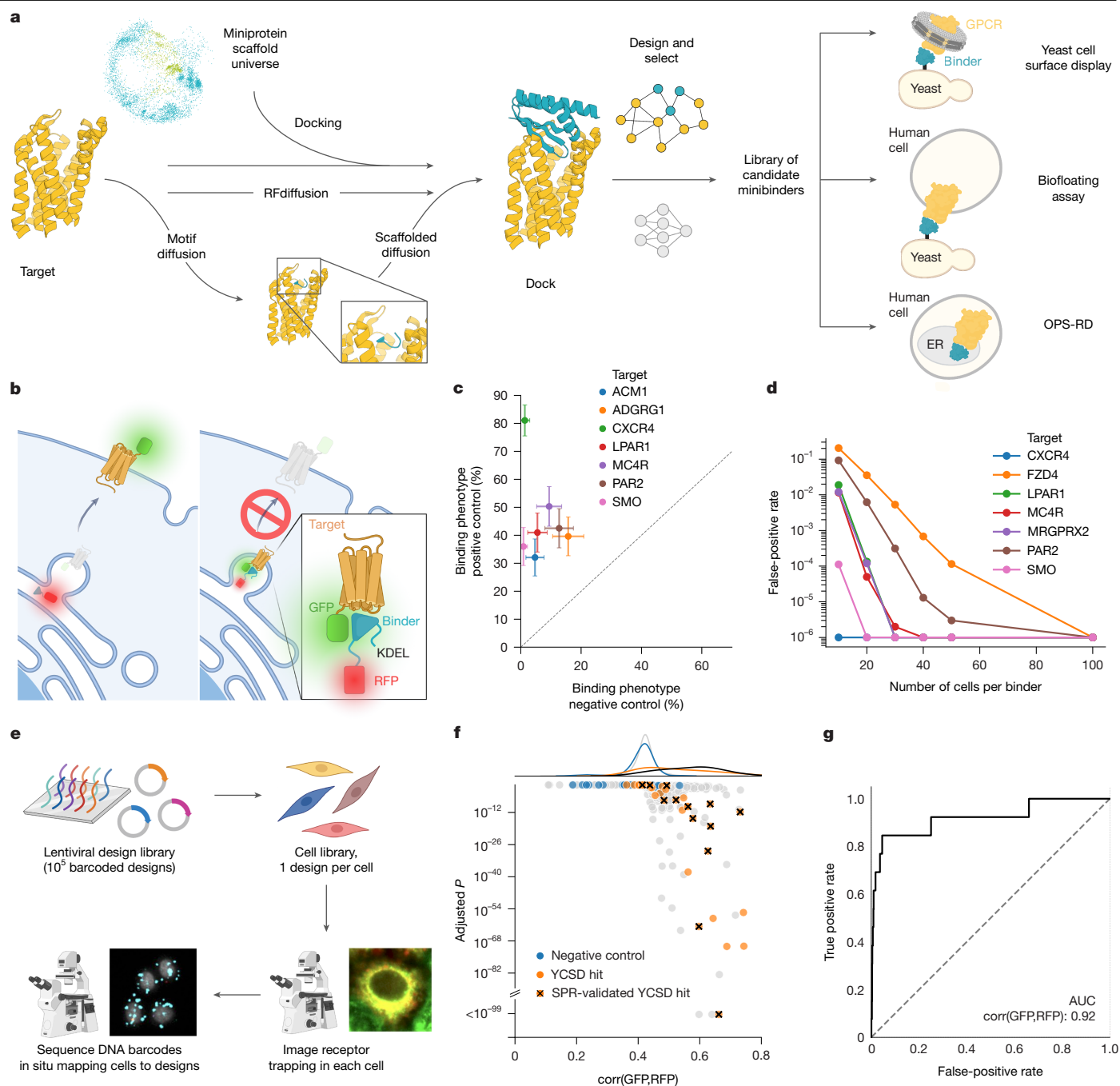
Fig. 1 | Computational design and screening of GPCR binders. a , Designed backbones targeting GPCRs were generated de novo by free or motif-guided RFdiffusion, or by docking 7,000 metaproteome-derived miniproteins. After sequence assignment and in silico prioritization, class A and B GPCR designs were screened in functional assays or by high-throughput binding assays, including yeast-surface display with soluble receptors, biofloating assay and OPS-RD. b , OPS-RD converts binder–receptor interactions into an optical phenotype. Without binding, fluorescently tagged receptors traffic to the cell surface while the design is retained separately in the secretory pathway. After binding, ER-retained binders trap fluorescently tagged wild-type receptors, causing colocalization in the secretory pathway. c , Across seven GFP-fused GPCRs, positive controls (oligomerized 0.7 nM anti-GFP nanobody LaG-16) produced significantly higher binding signals compared with the negative controls (non-binding miniproteins). The fraction of cells with the binding phenotype was calculated from at least 80 cells, and the s.e.m. was scaled to n = 50 cells, compatible with high-throughput screening. d , False-positive rate
